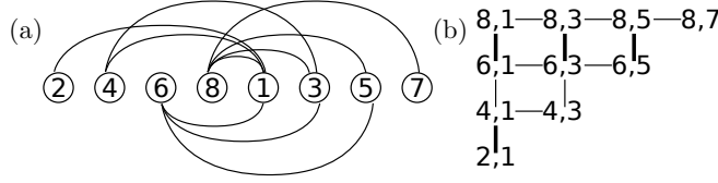
FIG. 2.1. (a) PG([2 4 6 8 1 3 5 7]) (b) A_{[2 4 6 8 1 3 5 7]}^a . Bold edges are those of the maximum matching M = \{\{(6,1), (8,1)\}, \{(6,3), (8,3)\}, \{(6,5), (8,5)\}, \{(2,1), (4,1)\}\} , the set of unmatched vertices is U = \{(4,3), (8,7)\} . The first short block-move is obtained by searching for the rightmost possible move involving pairs in M or vertices in U , for instance we take the pair (6,1), (8,1) applying the hop [2 \ 4 \ \underline{6} \ \underline{8} \ 1 \ 3 \ 5 \ 7] \rightarrow [2 \ 4 \ 1 \ 6 \ 8 \ 3 \ 5 \ 7] . Hence, we continue the search in M and U .
