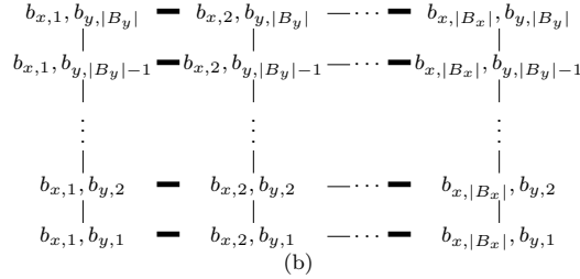
FIG. 3.3. G(B_x, B_y) . Bold edges represent the matching when: (a) |B_x| is even. (b) |B_x| is odd and |B_y| is even.
