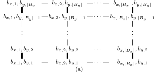
FIG. 3.2. Grid graph G(B_x, B_y) .
