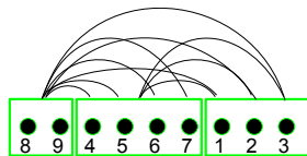
FIG. 3.1. The permutation graph of [8\ 9\ 4\ 5\ 6\ 7\ 1\ 2\ 3] . There are arcs between all elements in a block of adjacencies on the left and all elements in a block of adjacencies on the right.
